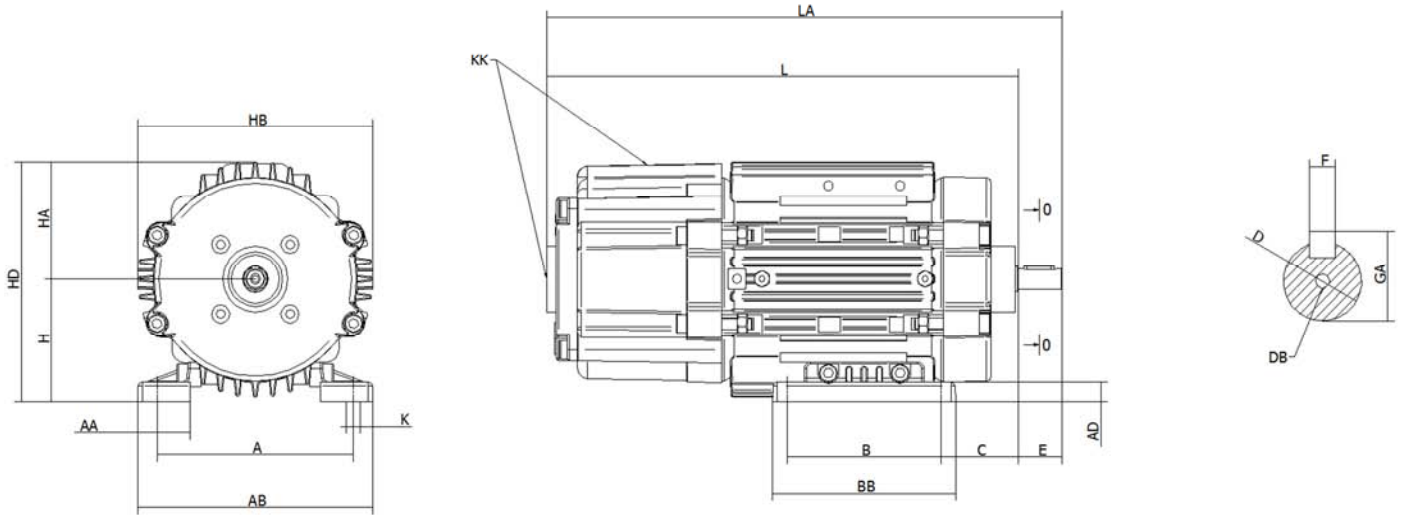
Mounting B3
