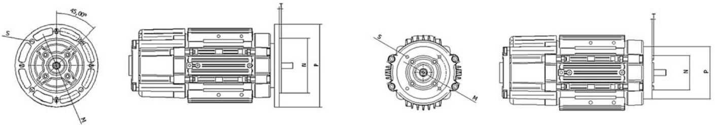
Mounting B3
