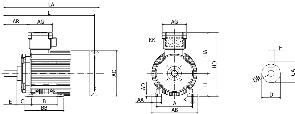
Mounting B3
