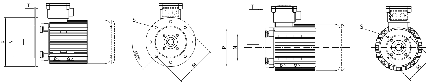
Mounting B5 4 (8) holes - 45°
